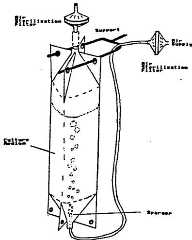
FIGURE 1 SMALL FERMENTER
